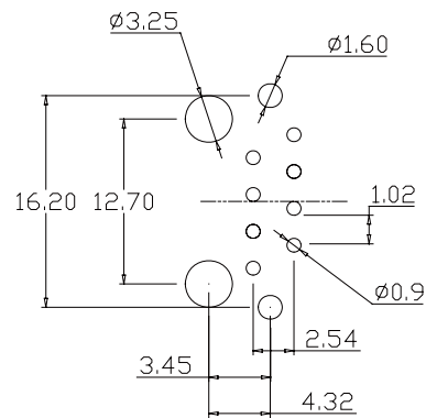
Recommended PCB Layout (PCB TOLERANCE \pm 0.05 )
